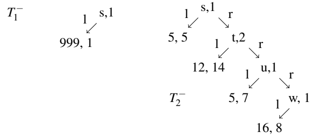
Figure 4: The maximum pay-off restricted trees corresponding to the trees in Fig. 3.
