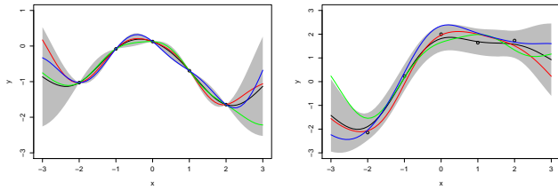
(a) No observation noise. (b) With uniform, uncorrelated Gaussian noise ( \sigma^2 = .1 ).
